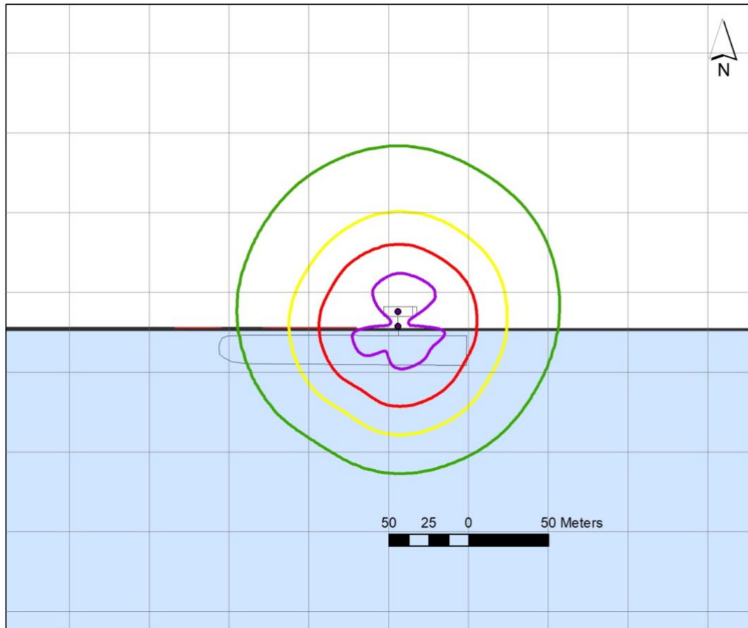
Figure 9. Location-related risk contours (1) stand-alone LNG (single tank truck)
